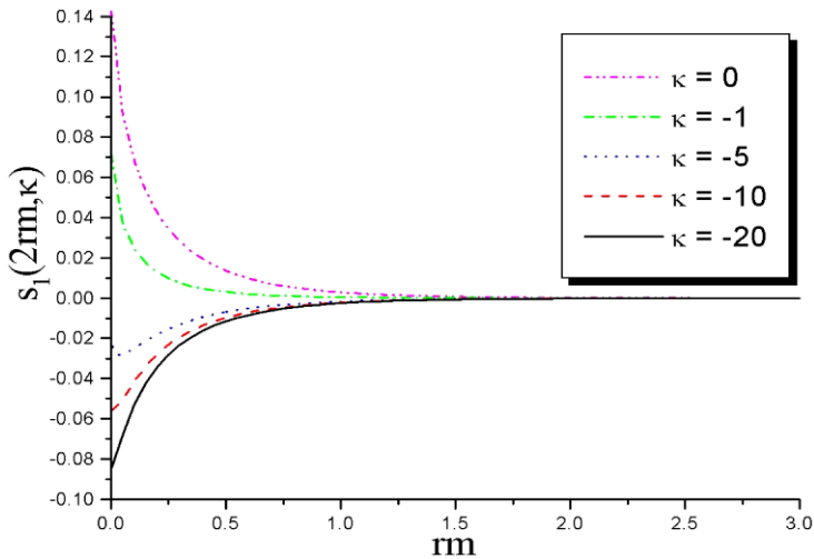
Fig. 1 The function s_1(2rm, \kappa) for several values of \kappa
