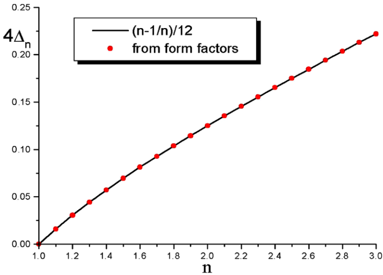
Fig. 4 The exponent in the short-distance behaviour of the bulk two-point function, as function of the number of sheets n analytically continued to n \geq 1 . This should be twice the scaling dimension, and the curve shows the expected value from CFT. The data points come from a re-summation of about 30 terms in the form factor expansion for the logarithm of the two-point function. For n > 2 , an improvement using Euler’s formula is needed in order to make the series convergent
