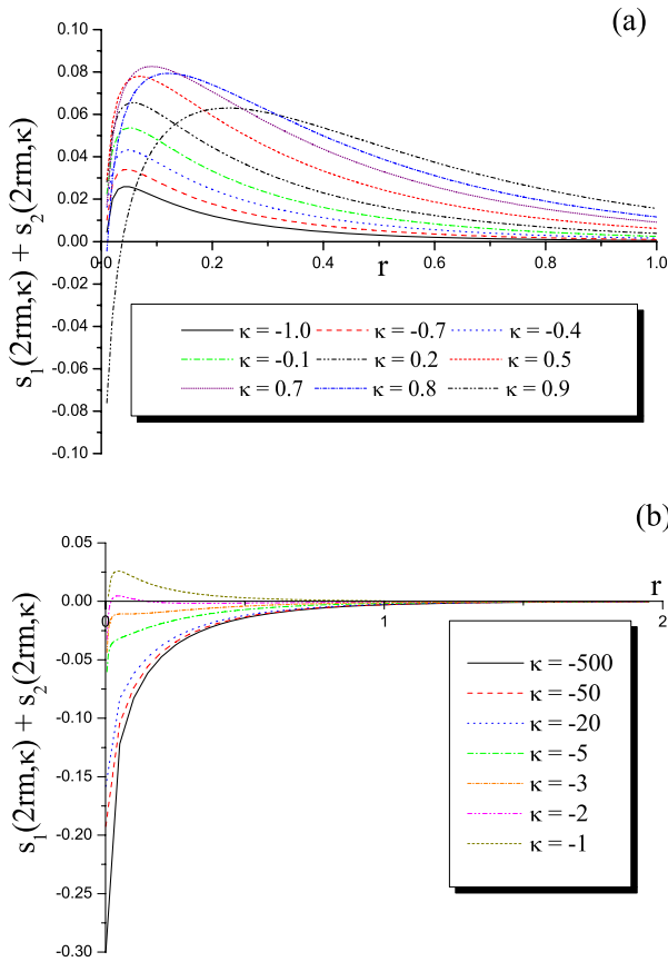
Fig. 2 The function s_1(2rm, \kappa) + s_2(2rm) for 0 < r \leq 2 . The value of rm for which the entropy is maximal for a given value of \kappa increases as \kappa gets closer to 1. As in Figs. 2(a) and 2(b), the maximum of the entropy seems most pronounced for \kappa = 0.7 and rm around 0.1 and tends to shift and eventually disappear as \kappa \rightarrow 1 . However, since the maximum occurs generally for rather small values of rm , its position may be affected significantly by higher order form factor corrections. Moreover, for \kappa > 0 , additional contributions to s_2 may come from the boundary bound state. Yet, it is certain that there is a maximum for \kappa \geq -1 as in this case the function tends to zero from above as rm \rightarrow \infty
