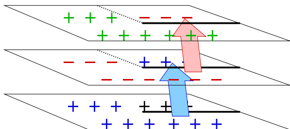
Fig. 3 How a vacuum of the form \dots \otimes |0, +\rangle \otimes |0, -\rangle \otimes |0, +\rangle \otimes \dots becomes a two-particle state after going through a branch-point twist field
